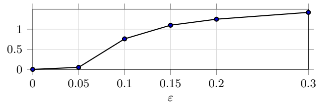
Fig. 5: Behavior of the cumulative discrepancy \sum_{k=1}^N \|y_{\text{LIN},k} - y_k\|_2^2 evaluated for increasing values of \varepsilon .
