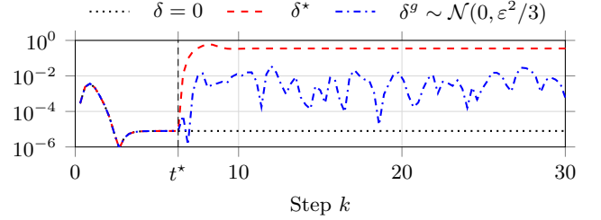
Fig. 4: Closed-loop error for \varepsilon = 0.15 under the optimized perturbation \delta^* and a Gaussian perturbation \delta^g \sim \mathcal{N}(0, \varepsilon^2/3) , activated at time t^* .
