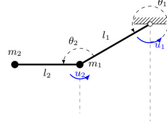
Fig. 3: Representation of the fully actuated double pendulum with state \mathbf{x} , joint torques as inputs, and joint angles as outputs.
