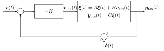
Fig. 2: Schematic representation of the closed-loop system perfectly linearized.
