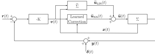
Fig. 1: Schematic representation of the closed-loop system linearized with an approximate model \tilde{\Sigma} corrected by a learning block.
