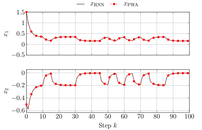
Fig. 3. Comparison between the state trajectories x_1, x_2 of RNN and CPWA dynamical system starting from the same initial condition and excited by the same input signal.
