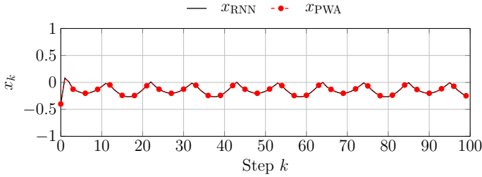
Fig. 4. Comparison between the state trajectories x_k of RNN and CPWA dynamical system starting from the same initial condition and excited by the same input signal.
