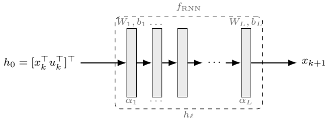
Fig. 1. Schematic of the recurrent neural network in Def. 2. The state x_k is propagated through L parameterized layers along with the input u_k to return the next state x_{k+1} .
