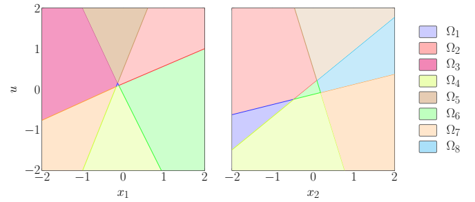
Fig. 2. Feasible regions of the ReLU RNN projected onto the planes (a) x_2 = 0 and (b) x_1 = 0 . Each color corresponds to a distinct activation pattern, i.e., a locally affine subsystem (Table 1). Borders are drawn in a darker shade of the same color as their region.
