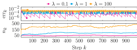
Fig. 1. Open ADMM applied to an unsupervised learning problem in an open network with \lambda^{\text{join}} = \lambda^{\text{leave}} = \lambda \in \{0.1, 1, 100\} .
