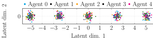
Fig. 2. Two-dimensional latent-space projection of the datasets for five randomly selected agents in the network at a random time during the simulation, under the worst-case configuration \lambda = 100 .
