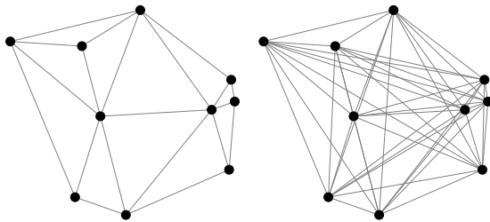
Fig. 2. Comparison between the number of arcs in the Delaunay graph (left) versus the complete graph (right).
