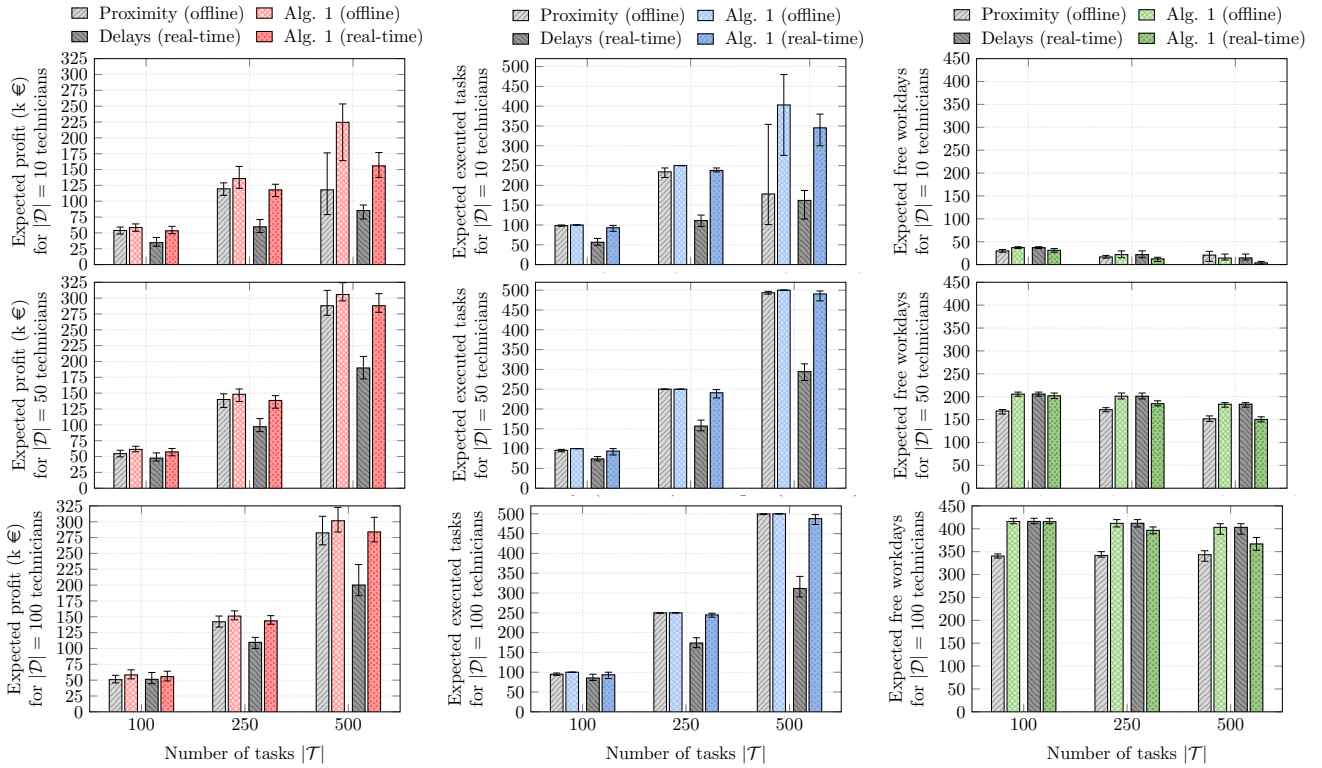
Fig. 5. Performance comparison of Algorithm 1 under offline and real-time conditions across synthetic problem instances with varying numbers of technicians and tasks. In the offline setting, “Proximity” denotes a baseline heuristic assigning tasks to the nearest technicians, serving as a warm start for Algorithm 1. In the real-time setting, “Delays” represents simulations incorporating stochastic task execution delays without any dynamic compensation logic, contrasted against Algorithm 1’s real-time dynamic reassignment, routing, and scheduling capabilities. The figure illustrates how Algorithm 1 consistently improves expected profit, the number of expected executed tasks, and the number of free workdays in static/dynamic environments.
